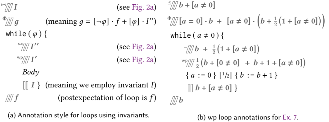
Fig. 3. Annotation style for loops using invariants and annotations for Ex. 7. Inside the loop, we push an invariant I (provided externally, denoted by \llbracket I ) through the loop body, thus obtaining I'' which is (possibly an over- or underapproximation of) \text{wp} \llbracket \text{Body} \rrbracket (I) . Above the loop head, we then annotate g = [\neg\varphi] \cdot f + [\varphi] \cdot I'' . In the first line, we establish g \bowtie I , for \bowtie \in \{\leq, \geq\} . Note that if \bowtie = \leq , we have established the precondition of Cor. 6, since we have then overall established
