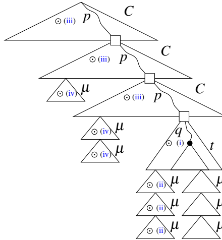
Figure 2: Leftmost redexes
